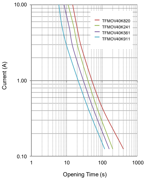
Limited Current Test Curve (UL 1449 clause 44.4)
